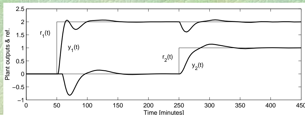
Figure 6.12: Simulation results for PI control of distillation column
